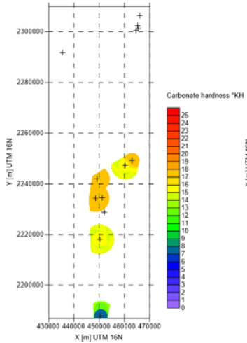
CECyTE Tulum water monitoring campaign spring 2017 - distribution of Carbonate hardness - week 23/2017
