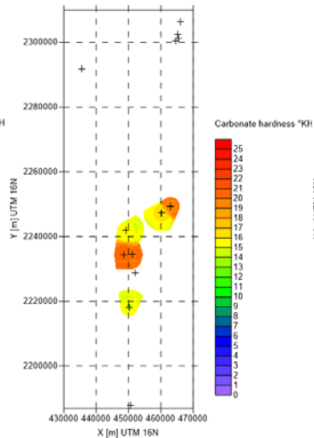
CECyTE Tulum water monitoring campaign spring 2017 - distribution of Carbonate hardness - week 25/2017
