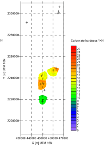
CECyTE Tulum water monitoring campaign spring 2017 - distribution of Carbonate hardness - week 24/2017
