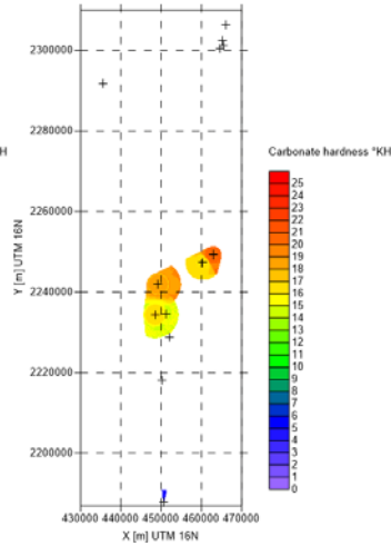
CECyTE Tulum water monitoring campaign spring 2017 - distribution of Carbonate hardness - week 19/2017
