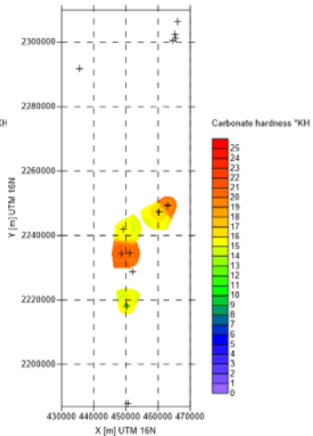
CECyTE Tulum water monitoring campaign spring 2017 - distribution of Carbonate hardness - week 26/2017
