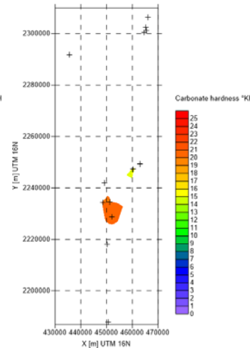
CECyTE Tulum water monitoring campaign spring 2017 - distribution of Carbonate hardness - week 27/2017
