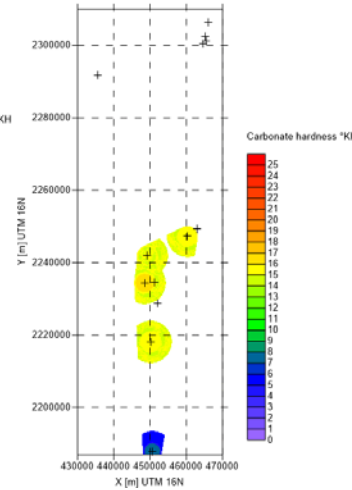
CECyTE Tulum water monitoring campaign spring 2017 - distribution of Carbonate hardness - week 22/2017
