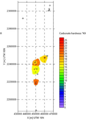
CECyTE Tulum water monitoring campaign spring 2017 - distribution of Carbonate hardness - week 20/2017
