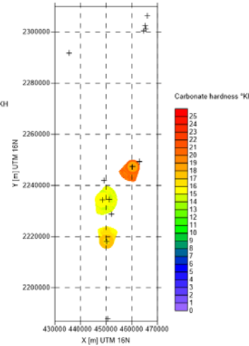
CECyTE Tulum water monitoring campaign spring 2017 - distribution of Carbonate hardness - week 21/2017
