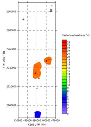
CECyTE Tulum water monitoring campaign spring 2017 - distribution of Carbonate hardness - week 18/2017
